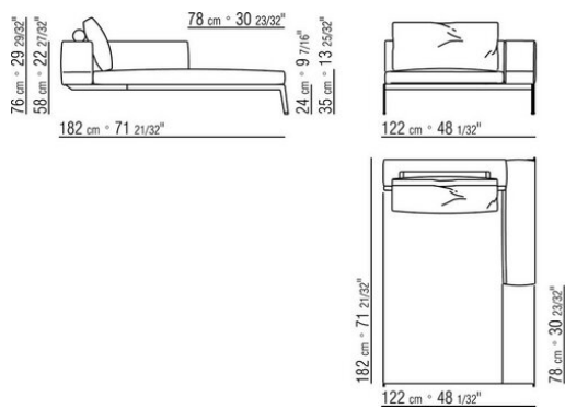
COD. 014C15
