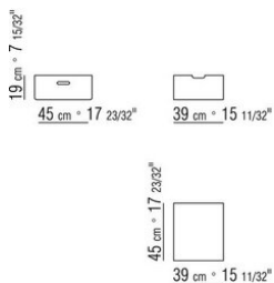
COD. 014X31
